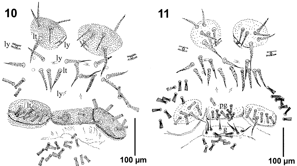
FIGURES 10–11. Salfacarus antsiranensis n. sp., sternitogenital region. 10, Female (OSAL007754); 11, Male (OSAL007765). lt: long, tapering setae; ly: lyrifissure (different types); pg: pregenital; g: genital.
