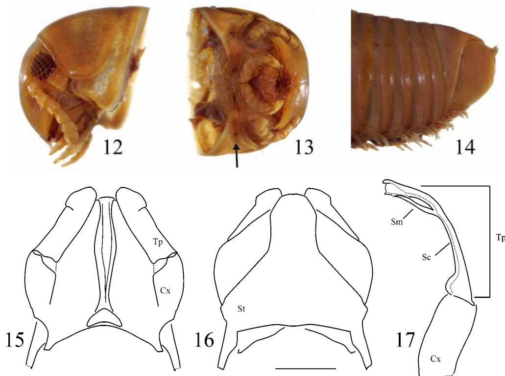
FIGURES 12–17. Oxygyge mesites (Chamberlin, 1922), male holotype. 12, lateral view of male anterior segments. 13, ventral view of anterior segments, arrow points to pits on first ring segment. 14, posterior segments, male. 15, anterior gonopod, posterior view. 16, anterior gonopod, anterior view. 17, left posterior gonopod. [Scale bar = 1.0 mm (Figs. 15–17)]
