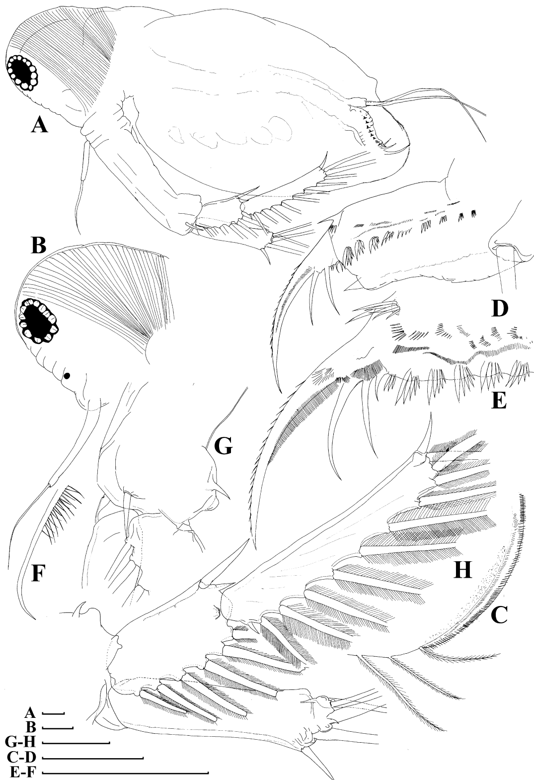
FIGURE 4. Pseudosida cf. szalayi (Daday, 1898), parthenogenetic female from Bak Sil Ji 3, locality 8. A, lateral view; B, head; C, postero-ventral portion of valve, inner view; D, postabdomen; E, its distal portion; F, distal sensory seta of antenna I; G, distal portion of basal segment of antenna II; H, branches of antenna II. Scale bars: 0.1 mm.
