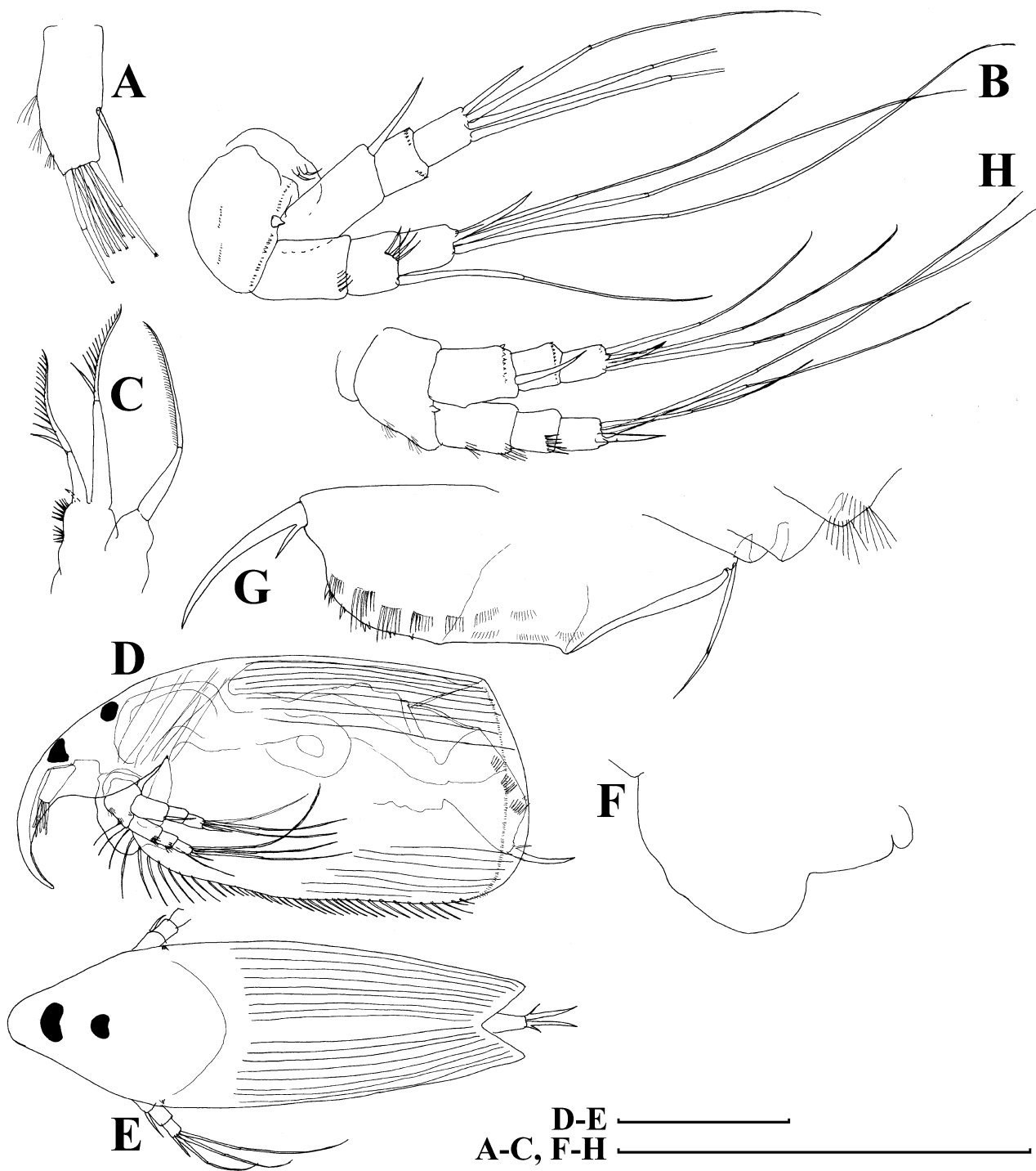
FIGURE 27. Nedorchynchotalona chiangi Kotov & Sinev, 2011, adult (A–C) and juvenile (D–H) parthenogenetic female from Bak Sil Ji I, locality 6a: A, antenna I of adult; B, antenna II; C, distal portion of limb I; D–E, juvenile, lateral and dorsal view; F, labrum; G, postabdomen; H, antenna II of juvenile. Scale bars: 0.1 mm.
