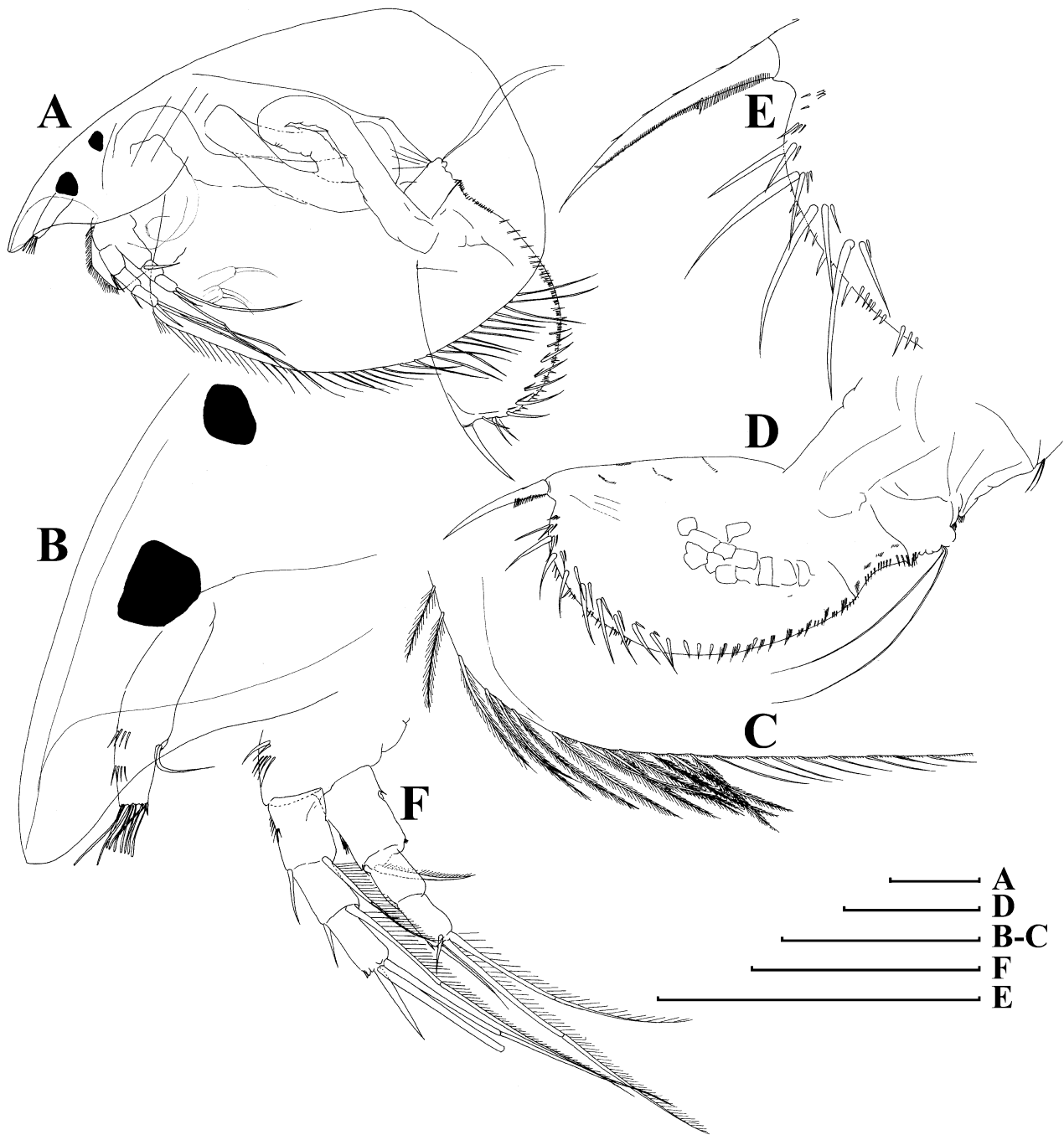
FIGURE 24. Leydigia (Neoleydigia) acanthocercoides (Fischer, 1854), parthenogenetic female from Bak Sil Ji 3, locality 8: A, lateral view; B, head; C, ventral margin of valve; D, postabdomen; E, its distal portion; F, antenna II. Scale bars: 0.1 mm.
