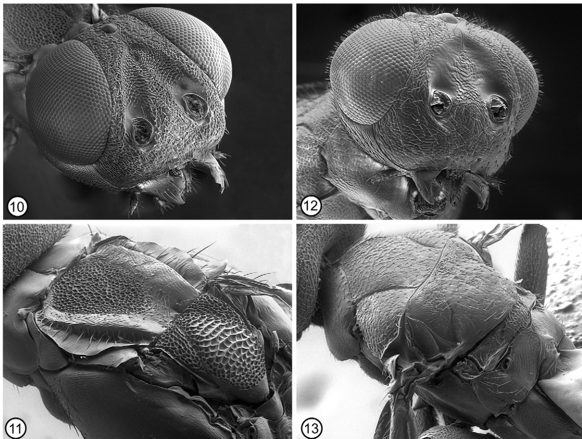
FIGURES 10–13. Anastatus eurycanthae Gibson (SEM). 10 , ♀ head, frontolateral view (2011-74); 11 , ♀ mesonotum, dorsolateral view (2011-74); 12 , ♂ head, frontolateral view (2011-81); 13 , ♂, mesosoma, dorsolateral view (2011-80).
