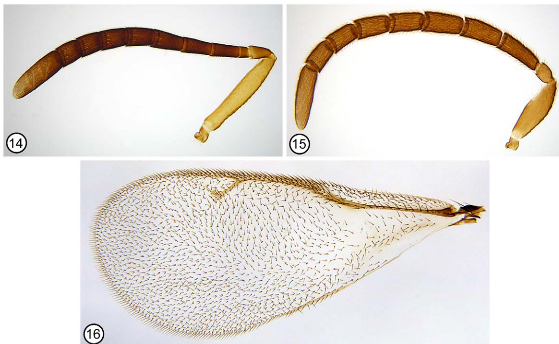
FIGURES 14–16. Anastatus eurycanthae Gibson (slide mounts). 14, ♀ antenna. 15, ♂ antenna. 16, ♂ fore wing.
