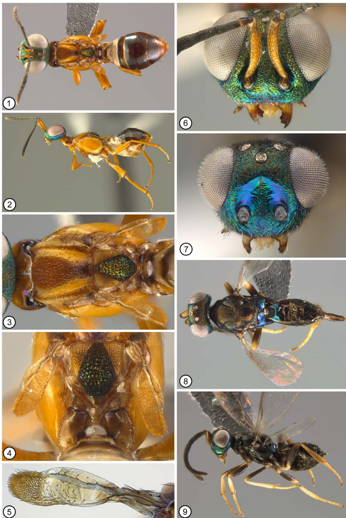
FIGURES 1–9. Anastatus eurycanthae Gibson. 1, ♀ dorsal habitus (2011-74); 2, ♀ lateral habitus (2011-75); 3, ♀ dorsal mesosoma (2011-75); 4, ♀ scutellar-axillar complex and propodeum (2011-74); 5, ♀ fore wing (2011-77); 6, ♀ head, frontal view (2011-74); 7, ♂ head, frontal view (2011-81); 8, ♂ dorsal habitus (2011-80); 9, ♂ lateral habitus (2011-79).
