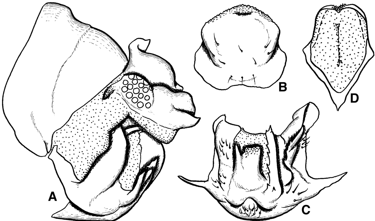
FIGURE 3. Male terminal structures of Trichadenotecnum sharkeyi . A: terminalia, lateral view; B: epiproct, posterodorsal view; C: hypandrium, posteroventral view; D: phallosome, ventral view.
