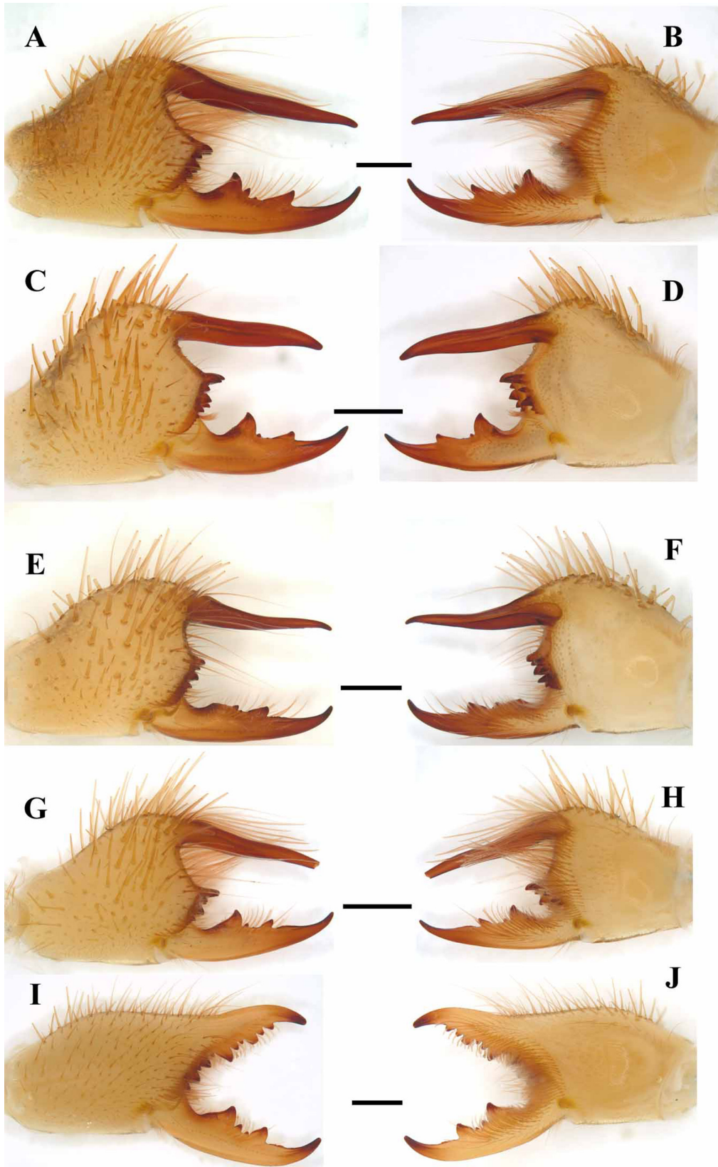
FIGURE 5. Retrolateral (left) and prolatral (right) cheliceral views of holotypes (and one allotype). Scale bars = 1.0 mm. A & B) Eremobates axacoa . C & D) Eremobates bonito . E & F) Eremobates cyranoi . G & H) Eremobates fisheri , male holotype. I & J) Eremobates fisheri , female allotype. K & L) Eremobates hidalgoana , female holotype. M & N) Eremobates jaliscoana . O & P) Eremobates minamoritaana . Q & R) Eremobates zacatecana . S & T) Eremobates zapal .
