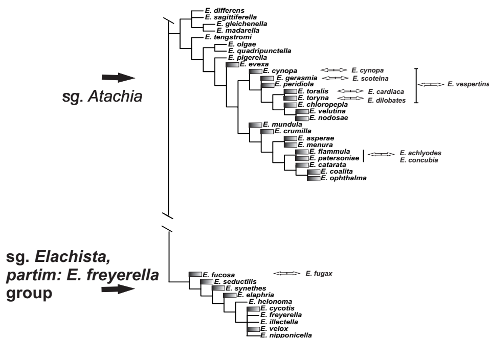
FIGURE 18. A cladogram showing the putative sister/vicariant species relationships between Australia and New Caledonia. The cladogram is modified from Kaila & Sugisima (2011). Species occurring in Australia are indicated by a flag-like symbol.
