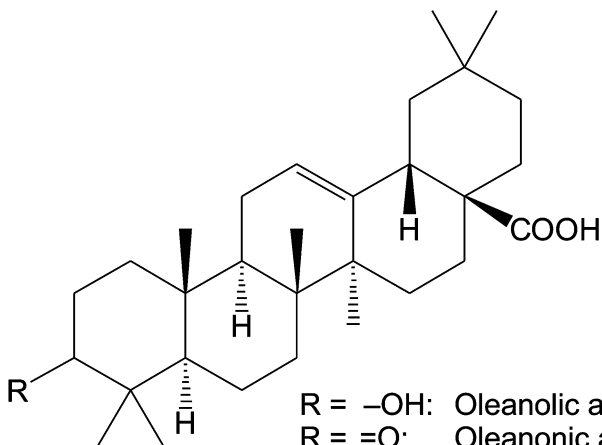
FIGURE 9. Chemical structure of the potential ingredients of styrax or storax resin from Liquidambar orientalis . Me, methyl.
