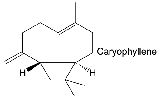
FIGURE 9. Chemical structure of the potential ingredients of styrax or storax resin from Liquidambar orientalis . Me, methyl.
