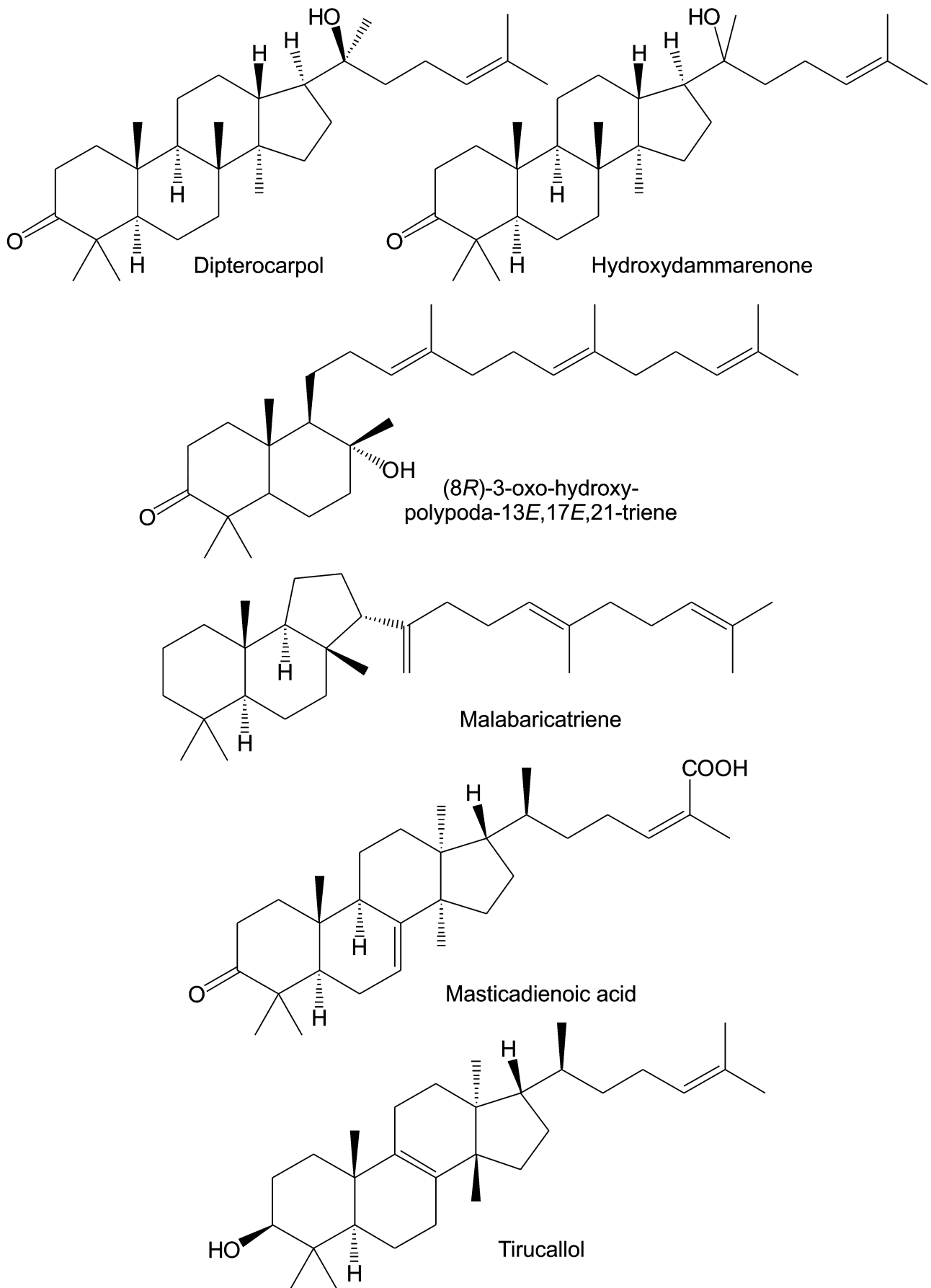
FIGURE 25. Chemical structure of triterpenes of gum mastic from Pistacia lentiscus , part 2.
