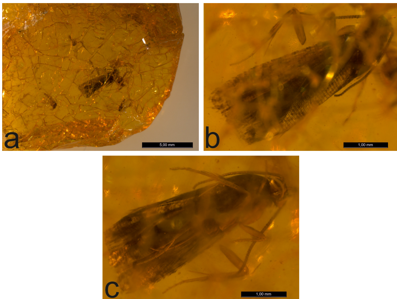
FIGURE 3. Electresia zalesskii Kusnezov, 1941. PIRAS (HT: no. 20). a. Crazing on the surface of the copal piece. b. Dorsal view. Length of forewing 4.2 mm. c. Ventral view. Photos: Maria Heikkilä.
