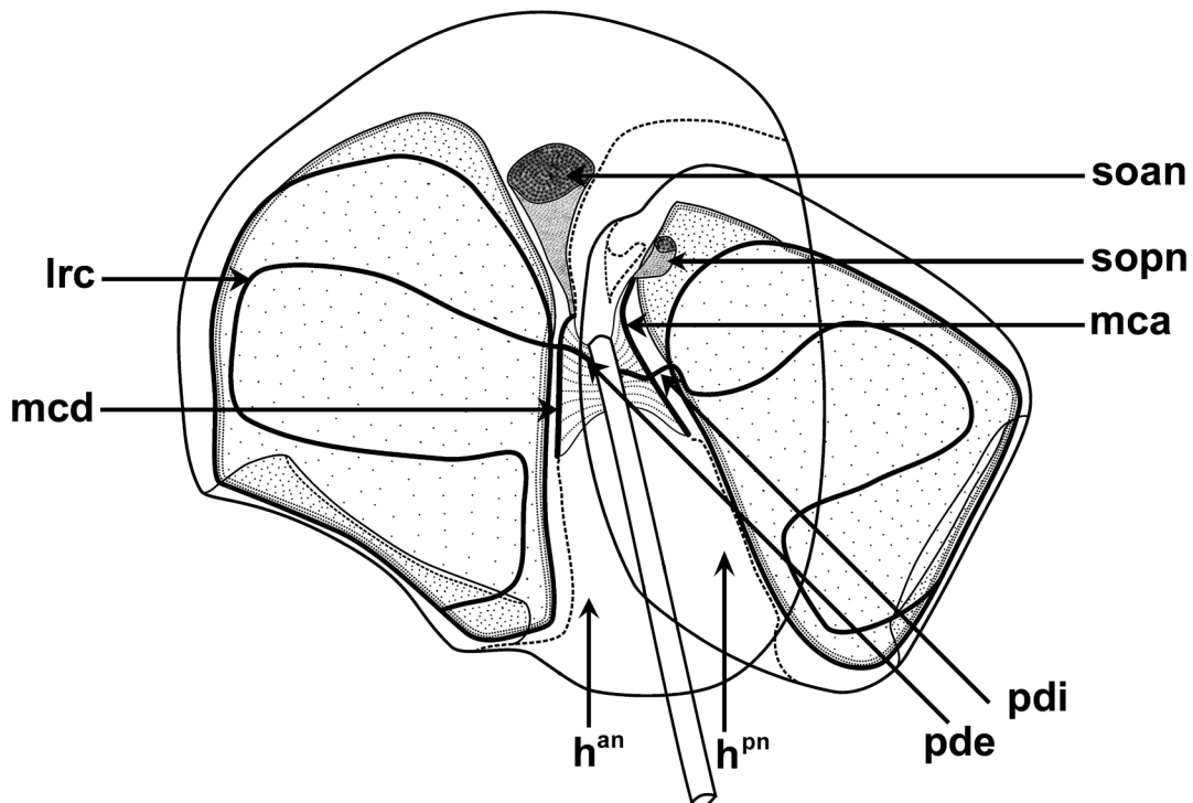
FIGURE 7. Nectophores of Tottonophyes enigmatica sp. nov. A. anterior, and B posterior. h an , h pn : hydroecium of anterior and posterior nectophore, respectively; mca , mcd , ascending and descending mantle canal, respectively; ns : nectosac; pde , pdi , external and internal pedicular canal, respectively; soan , sopn : somatocyst of anterior and posterior nectophore, respectively. Scale bar 2 mm.
