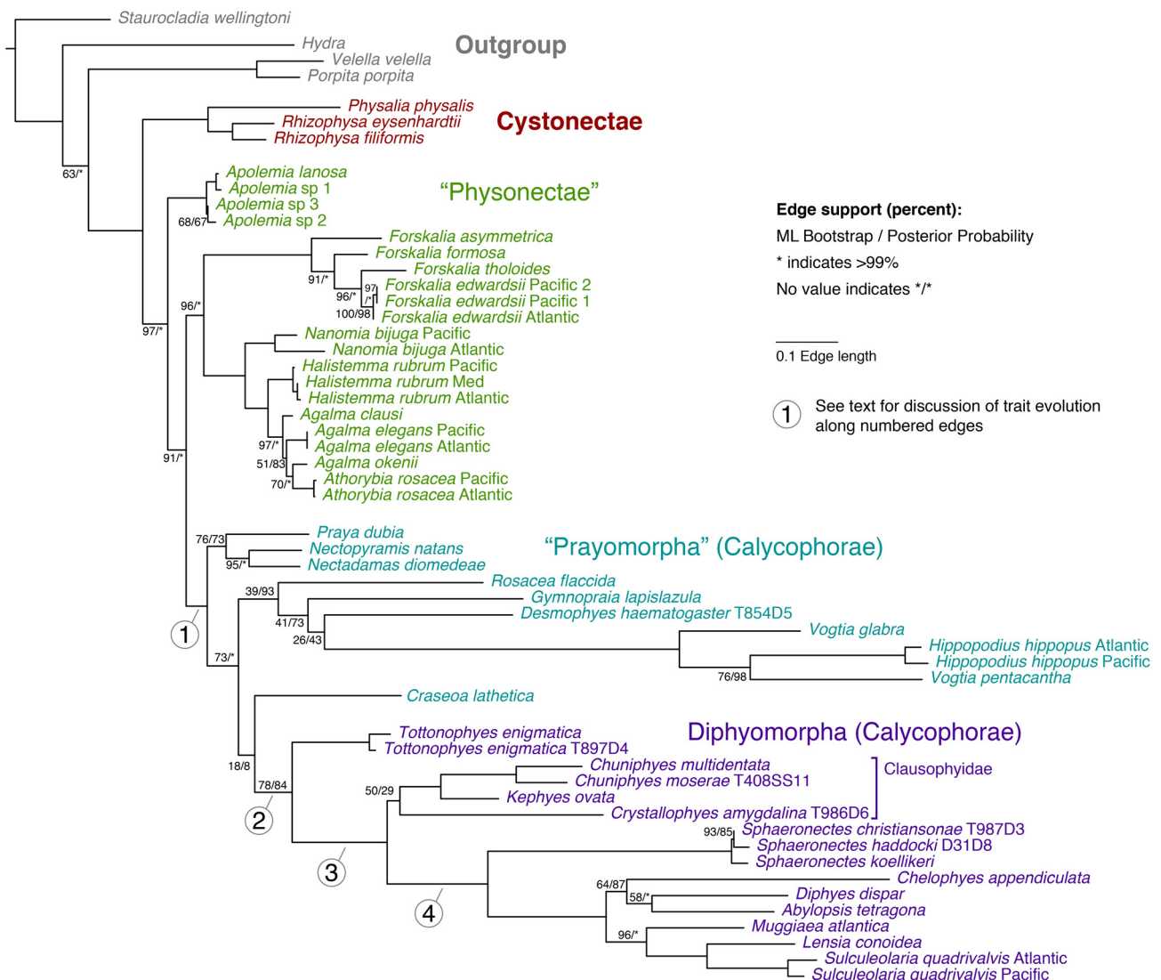
FIGURE 13. Phylogram of Siphonophora, including Tottonophyes enigmatica sp. nov. Bootstrap support values are shown at internal nodes. Unlabelled notes have 100/100 support. See methods for more information.
