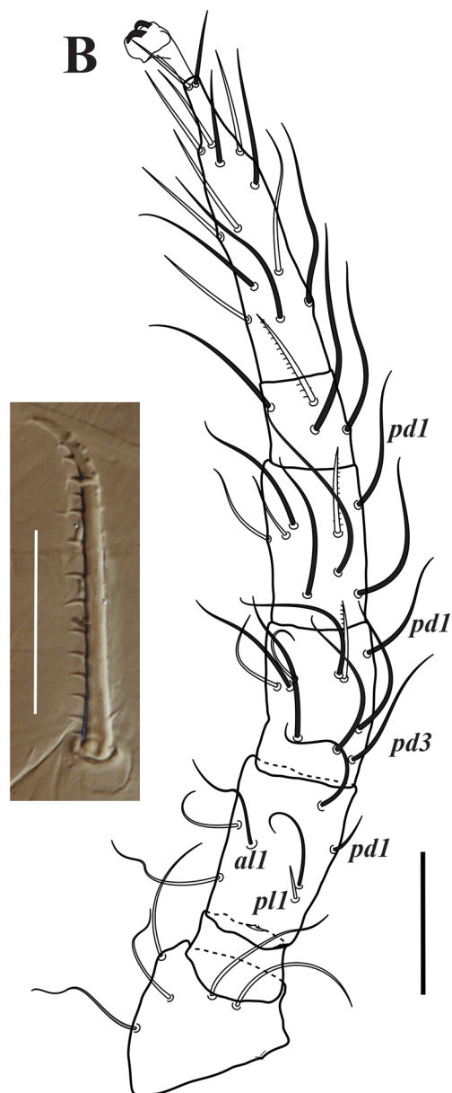
FIGURE 11. Philippinozercon makilingensis sp. nov., legs. A, Larva (OSAL 0052261), leg III; B, Deutonymph (OSAL 0053262), leg IV; inset: seta pl1 on genu. Scale bars legs = 100 \mu m, inset = 25 \mu m.
