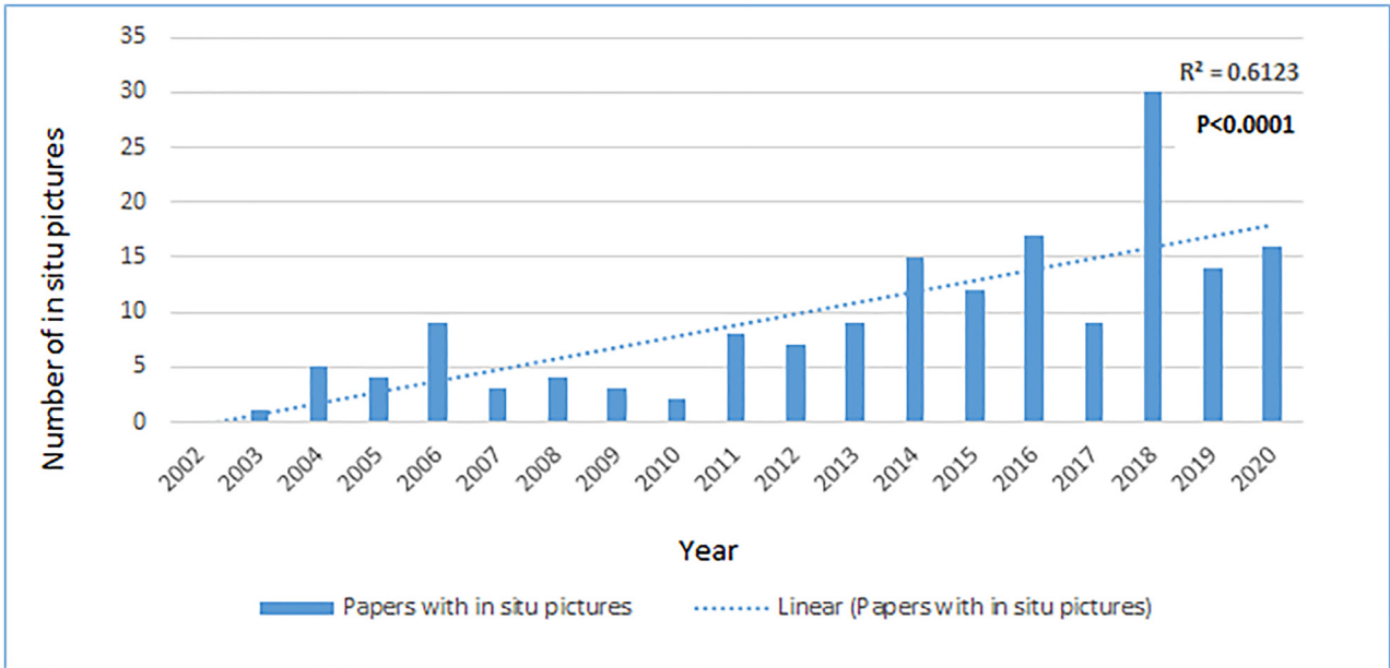
FIGURE 10. Number of papers with in situ illustrations of species of Porifera or their habitats published in Zootaxa each year between 2002 and 2020, with a linear regression trendline and analysis of the statistical significance of the observed data.
