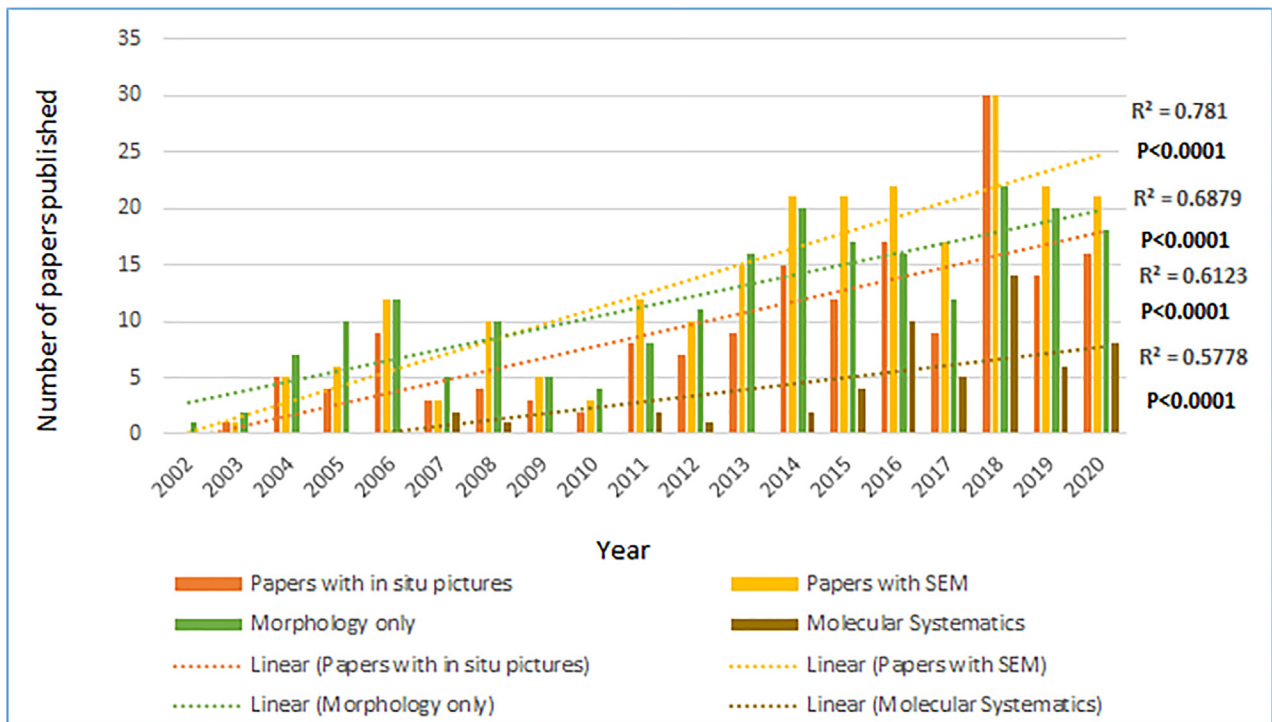
FIGURE 11. Number of papers with in situ illustrations of species or habitats (orange bars), scanning electron micrographs (SEMs, yellow bars), and including molecular systematics (brown bars), or based on morphology only (green bars), published on Porifera in Zootaxa each year between 2002 and 2020, with linear regression trendlines and analysis of the statistical significance of some of the observed data.
