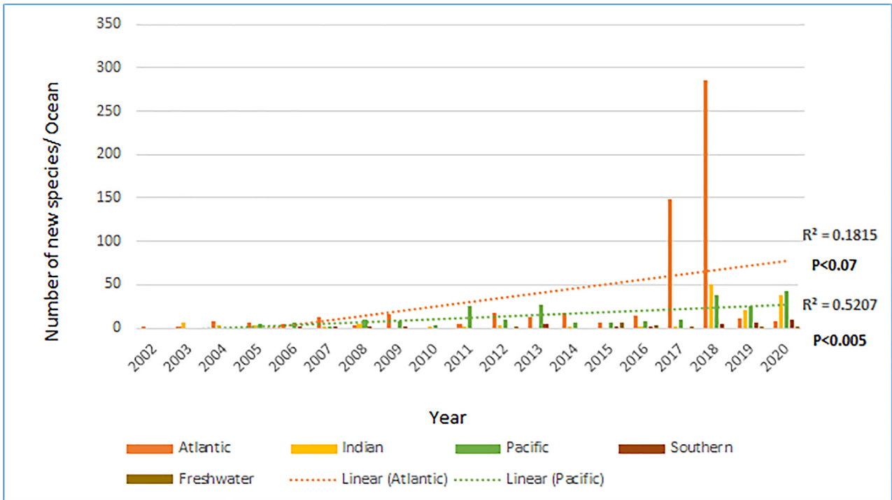
FIGURE 8. Number of new species per ocean basin (and freshwater bodies) published on Porifera in Zootaxa each year between 2002 and 2020, with linear regression trendlines and analysis of the statistical significance of the observed data for new species from the Atlantic Ocean (orange trendline) and new species from the Pacific Ocean (green trendline).
