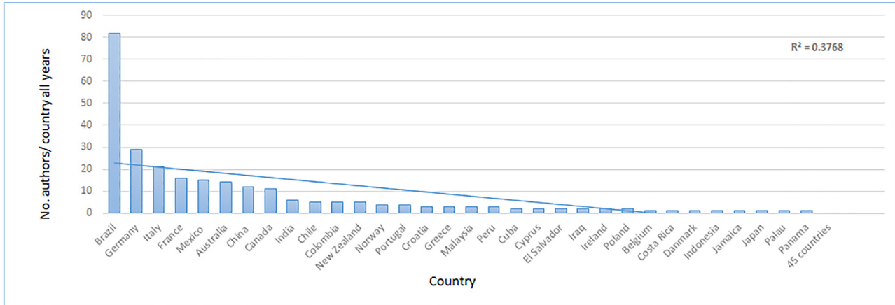
FIGURE 5. Number of authors in each country publishing on Porifera in Zootaxa each year between 2002 and 2020, with a linear trendline of the observed data.
