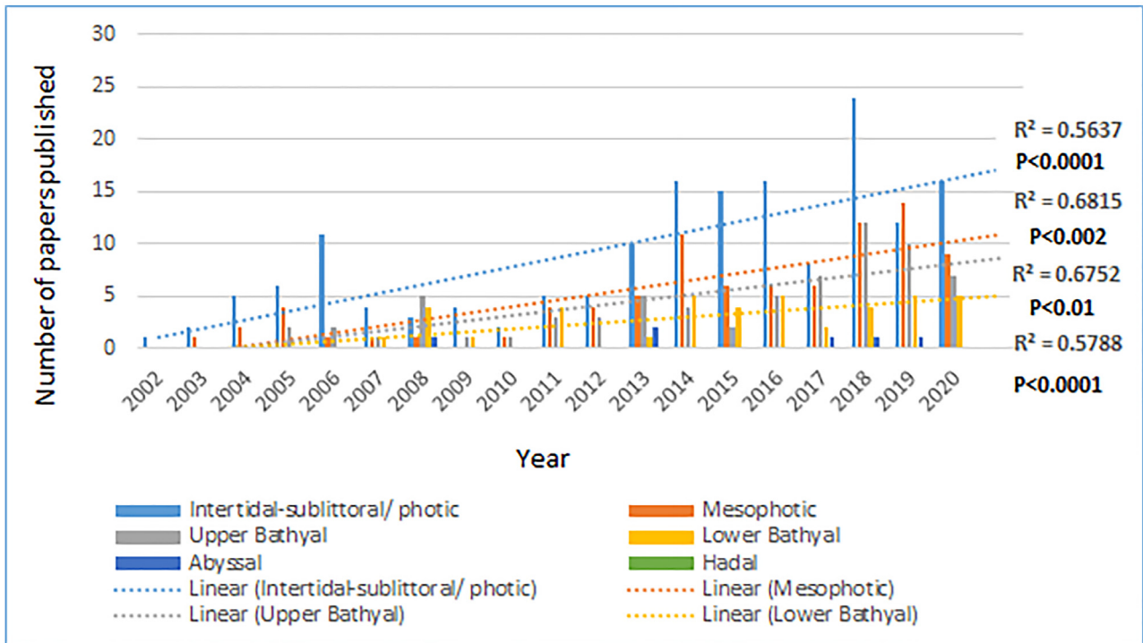
FIGURE 16. Number of papers published on Porifera in Zootaxa each year between 2002 and 2020 for each depth zone, with linear regression trendlines and analysis of the statistical significance of some of the observed data.
