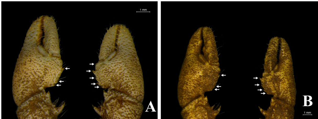
FIGURE 7. Aegla urussanga sp. nov. , Paraná 3 River Basin, Paraná, Brazil, MZUEL 545: A, juvenile male (CLE 12mm) MZUEL 525, dorsal view of palmar crest and chelipeds, white arrows indicate spines; B, juvenile female (CLE 11,75 mm) MZUEL 525, dorsal view of palmar crest and chelipeds, white arrows indicate spines. Scale = 1.0 mm.
