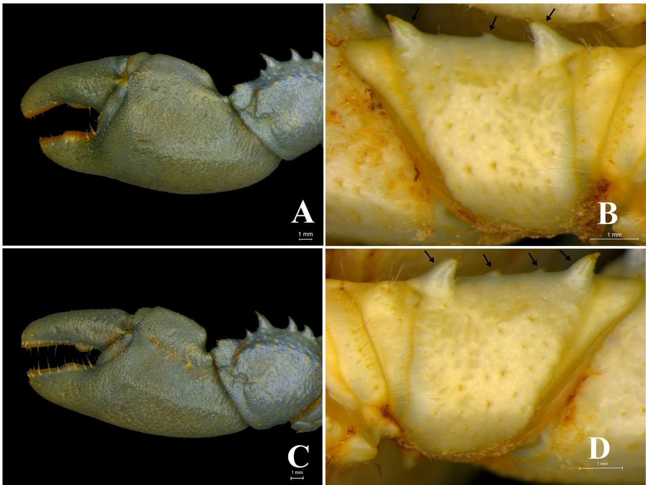
FIGURE 6. Aegla urussanga sp. nov., male holotype, CLE 22.0 mm, Paraná 3 River Basin, Paraná, Brazil, MZUEL 545: A, dorsal view of greater cheliped (left), rudimentary palmar crest; B, ventral view of the ischium of the greater cheliped (left) with two spines and one tubercle (black arrows); C, dorsal view of minor cheliped (right) showing rudimentary palmar crest; D, ventral view of the ischium of the minor cheliped (right) with two spines and two tubercles (black arrows). Scale = 1.0 mm.
