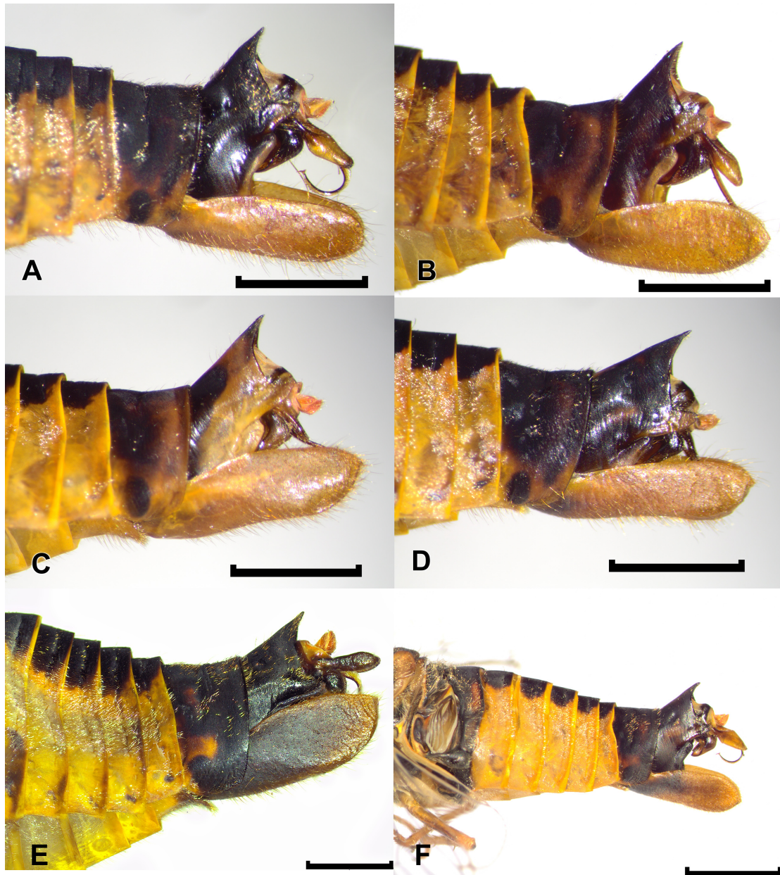
PLATE 3. Lateral views of male left abdomens: (A), Yoyetta darug sp. nov., Silverdale (33°52'S 150°37'E); (B), Y. darug sp. nov., Lake Parramatta, NSW (33°47'S 150°01'E); (C), Y. psammitica sp. nov., Windamere Dam, (32°43'S 149°46'E); (D), Y. psammitica sp. nov., Cassilis rest area (32°02'S 149°56'E); (E), Y. fumea sp. nov., Tarago (35°05'S 149°54'E 149°02'E); (F), Y. humphreyae , Blaxland (33°44'S 150°37'E). Scale bars = 5mm.
